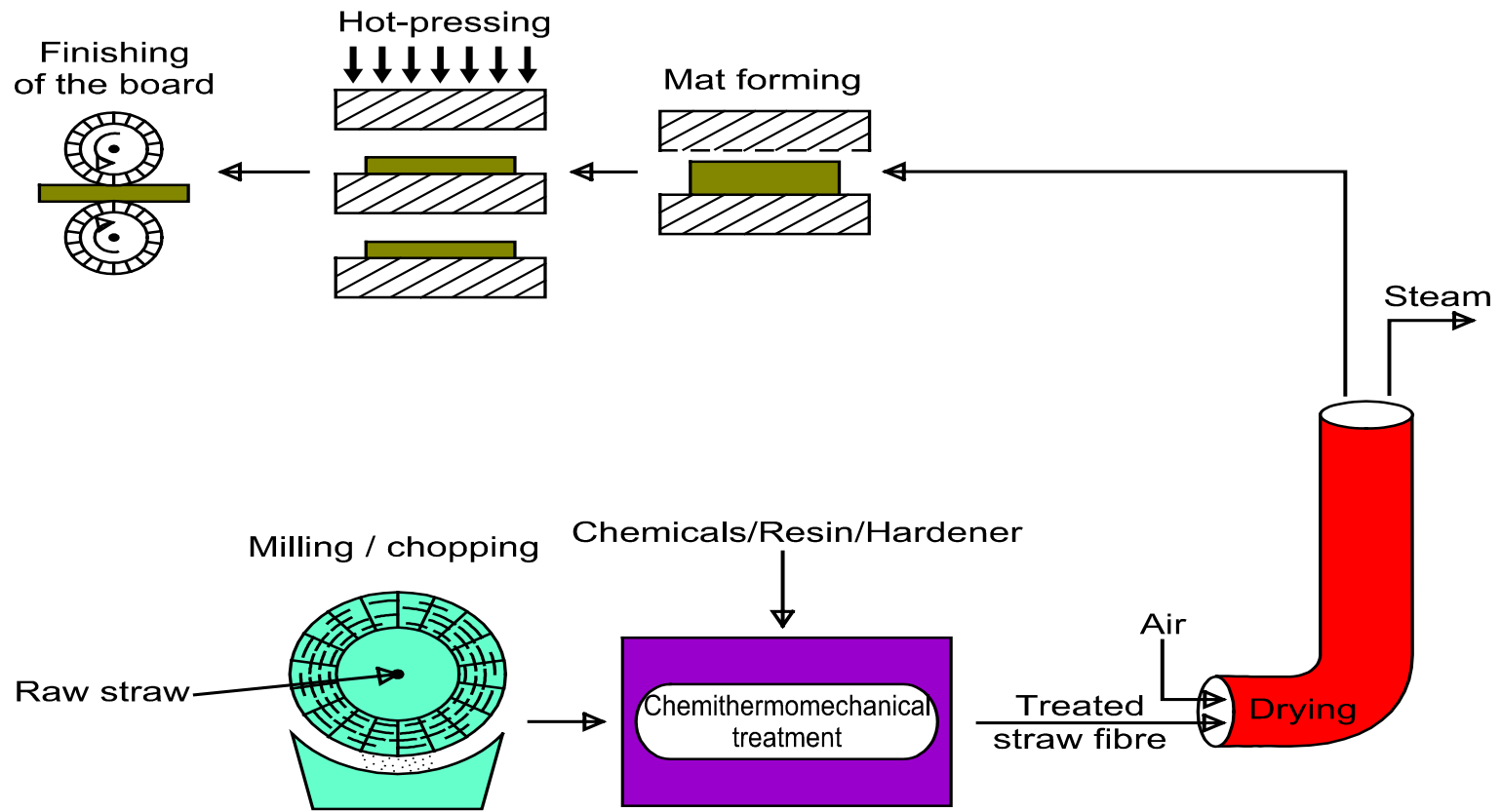
FIGURE 1. Schematic diagram of the strawboard production incorporating the new process.
